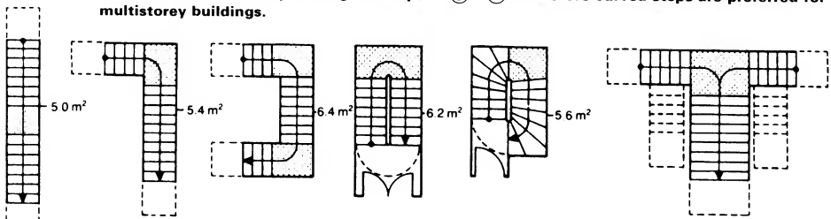
12 - 16 Stairs with landings take up the area of one flight of stairs + the surface area of landing - surface area of one step. For a height per storey of ≥ 2.75m, stairs with landings are necessary. Width of landing ≥ stair flight width.
